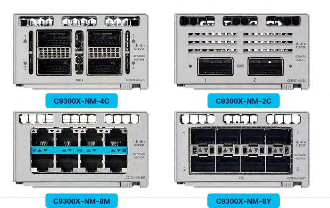
Figure 2. Cisco Catalyst 9300X Network Modules
