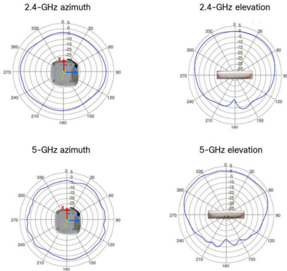
Figure 1. Antenna Profiles Diagrams
