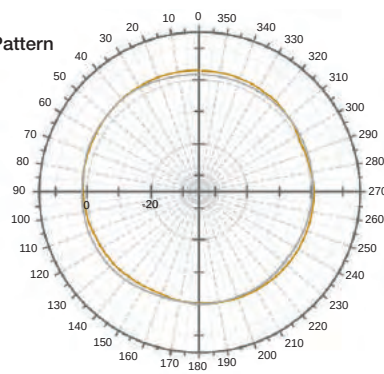
E-Plane Pattern
