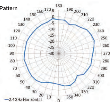
E-Plane Pattern
