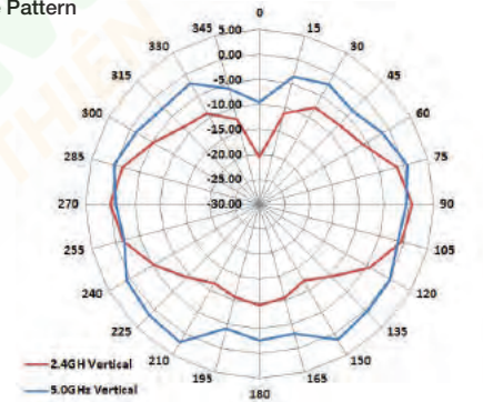
E-Plane Pattern
