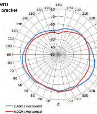
H-Plane Pattern with plastic wall bracket
