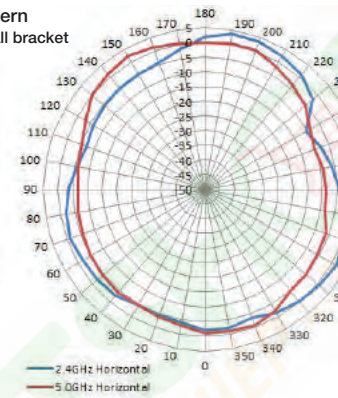
E-Plane Pattern with plastic wall bracket
