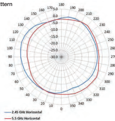
E-Plane Pattern
