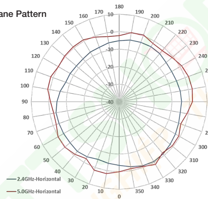
E-Plane Pattern
