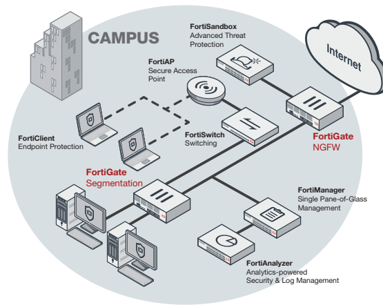
FortiGate 6300F/6500F deployment in large campus networks (NGFW, Intent-based Segmentation)
