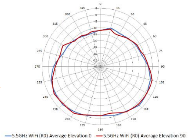
5.5GHz Wi-Fi antenna patterns (vertical)
