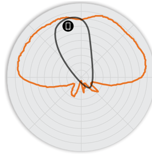
Figure 4. E510 2.4GHz Elevation Antenna Patterns
