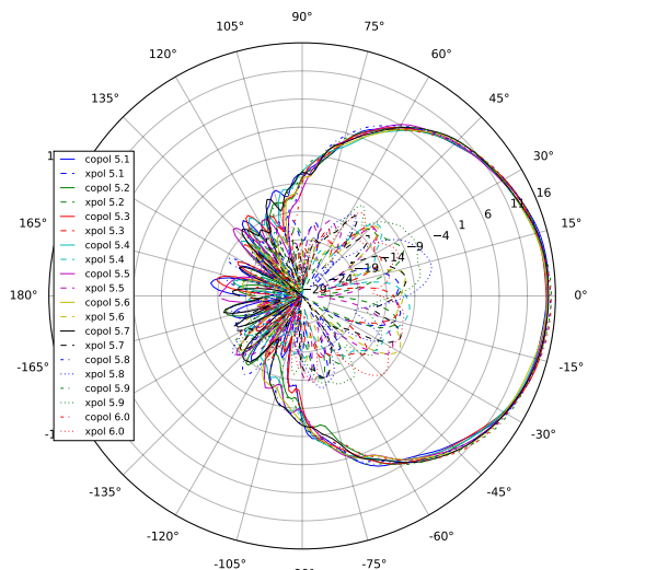
Sector Azimuth
