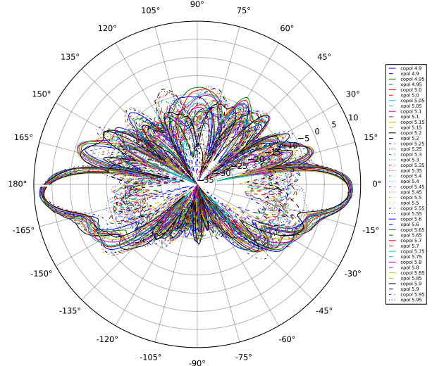
Omni Elevation
