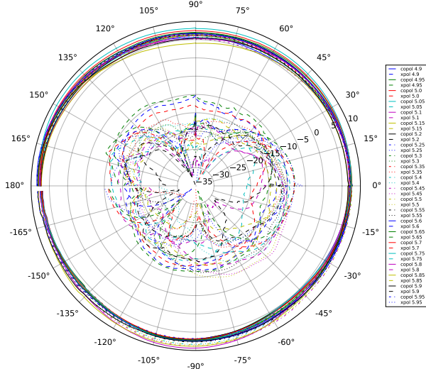
Omni Azimuth
