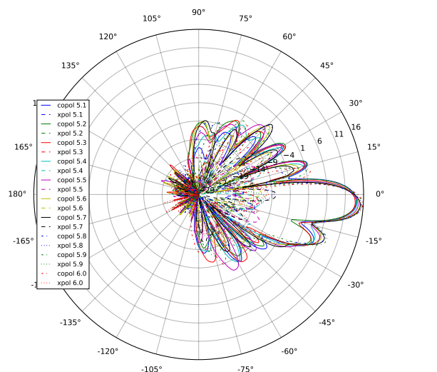
Sector Elevation
