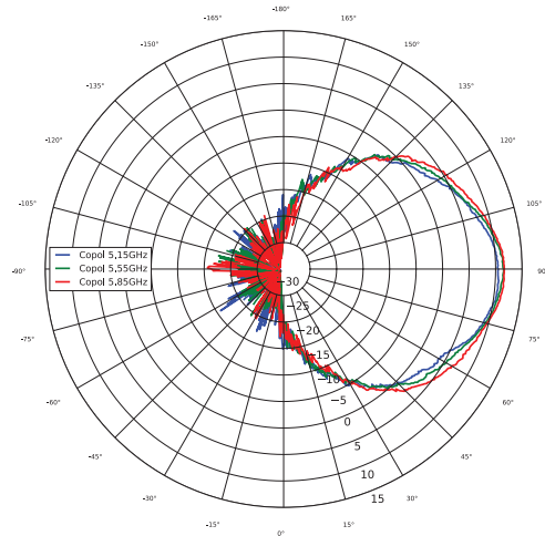
Channel 2 Vertical Polarization Elevation
