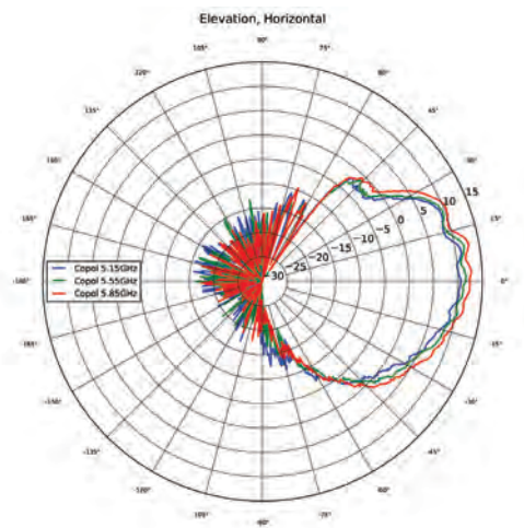
Channel 3 Horizontal Polarization Elevation
