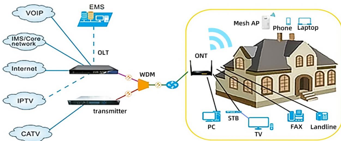
Picture 1-1 GN41AC products Network diagram
