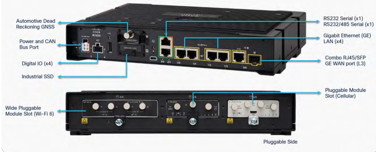
Figure 6. IR1835-K9 interface ports
