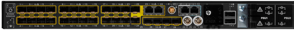
Figure 3. IE-9320-22S2C4X Switch with conformal coating and advanced feature set, including support for GPS/IRIG-B input
