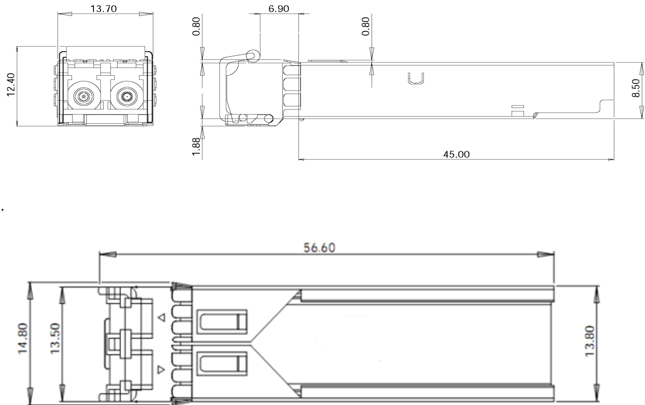
SFP-1G-10KM
